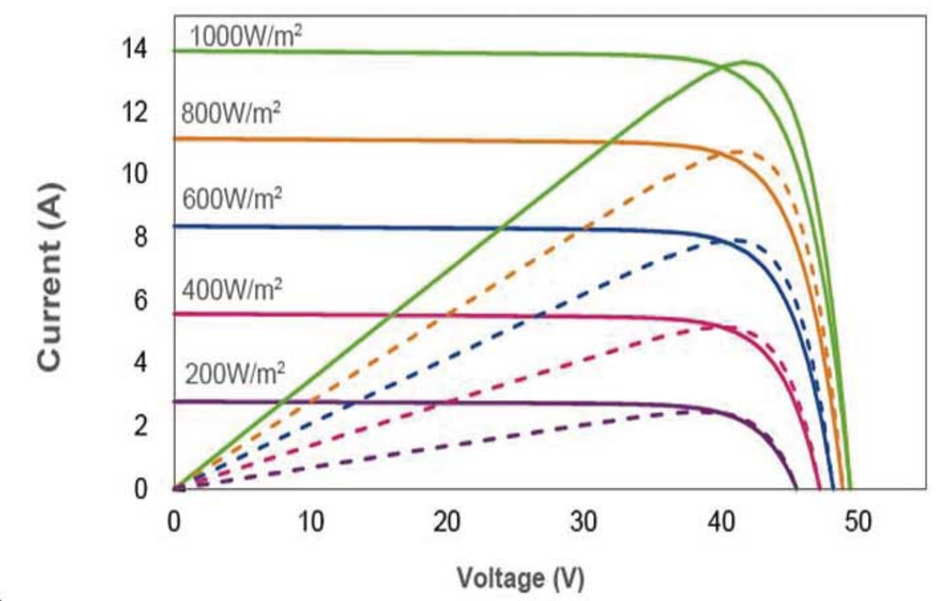
Current-Voltage Curve under different irradiance
