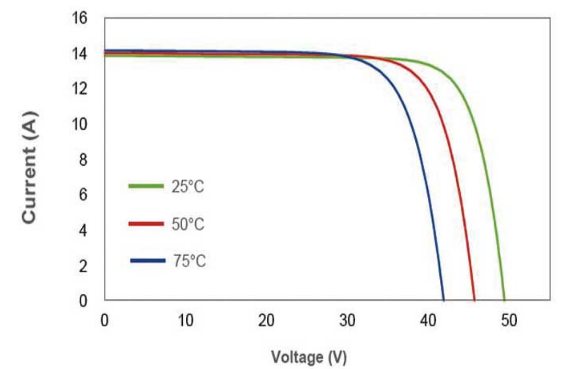
Current-Voltage Curve under different working temperatures
